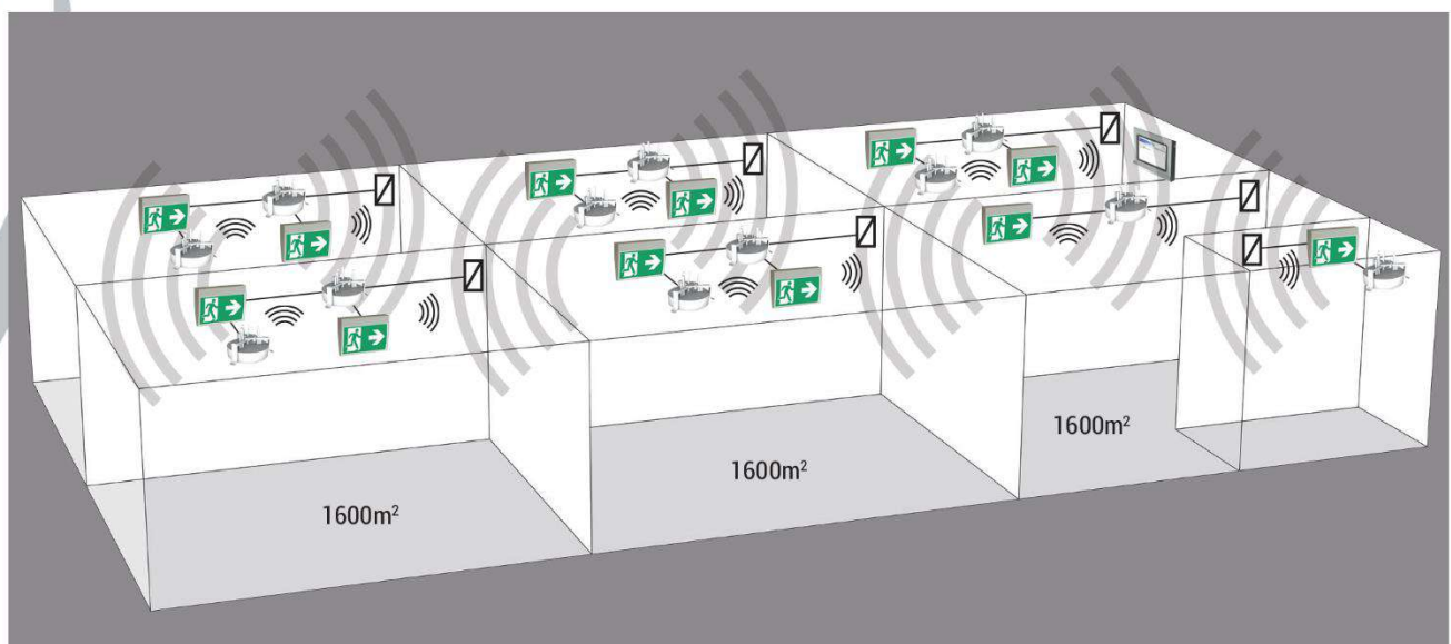
Example of an industrial hall with virtual fire zones
