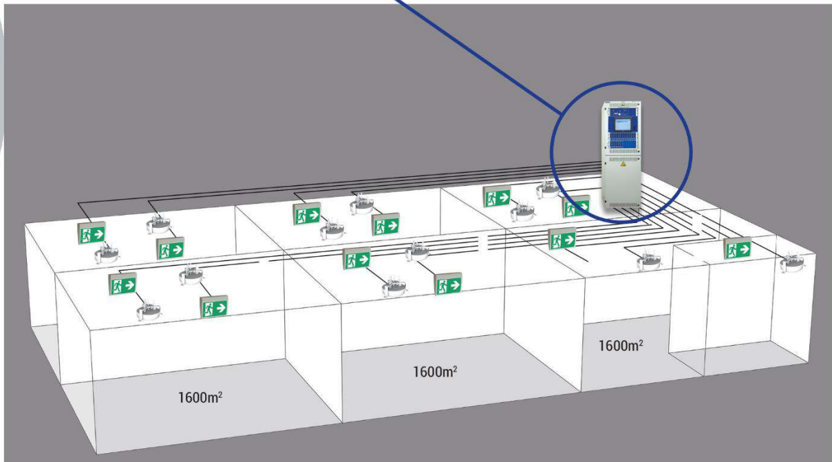
Power supply installation, as e. g. multiControl plus
